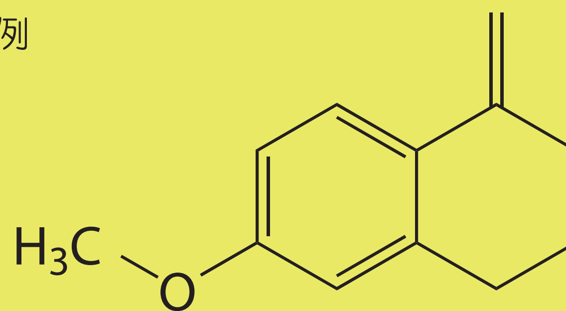
6-Methoxy 1-tetralone
