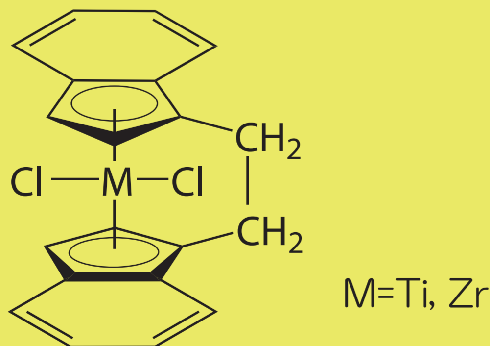
rac-Ethylenebis(1-indenyl)-metal dichlorides
