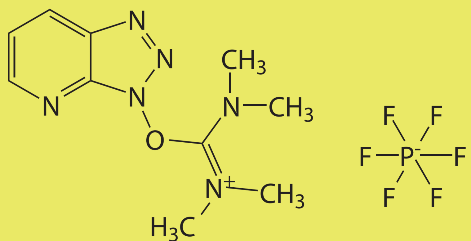
O-HATU (ペプチド試薬) o-(7-AZABENZOTRIAZOL-YL)-N,N,N', N'-TETRAMETHYL URONIUM HEXAFLUORO PHOSPHATE
