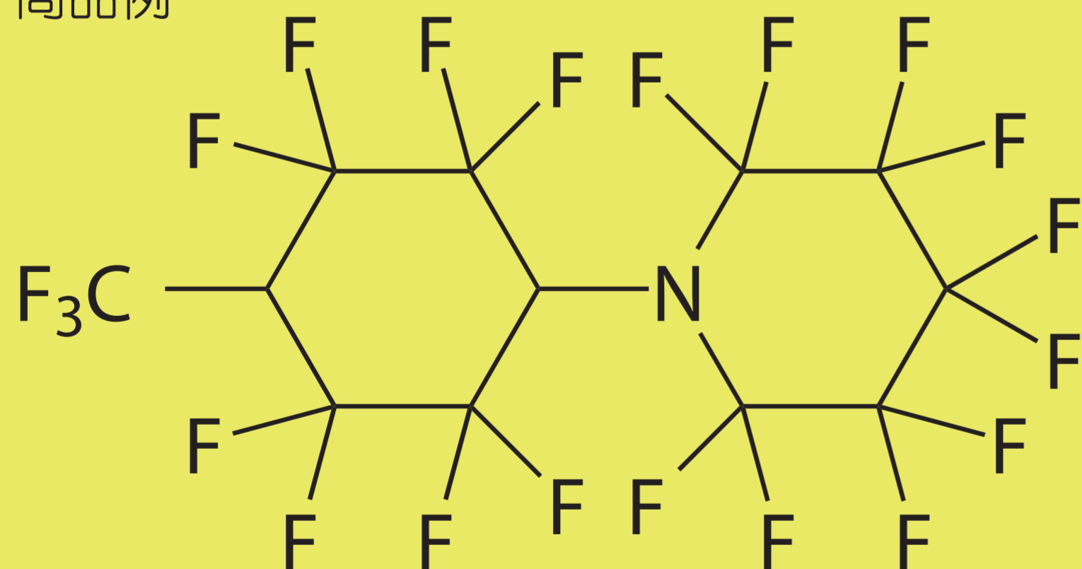
Perfluoro-N-(4-methyl-cyclohexyl) piperidine (PMCP)
