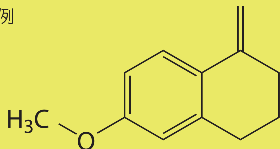
6-Methoxy 1-tetralone
