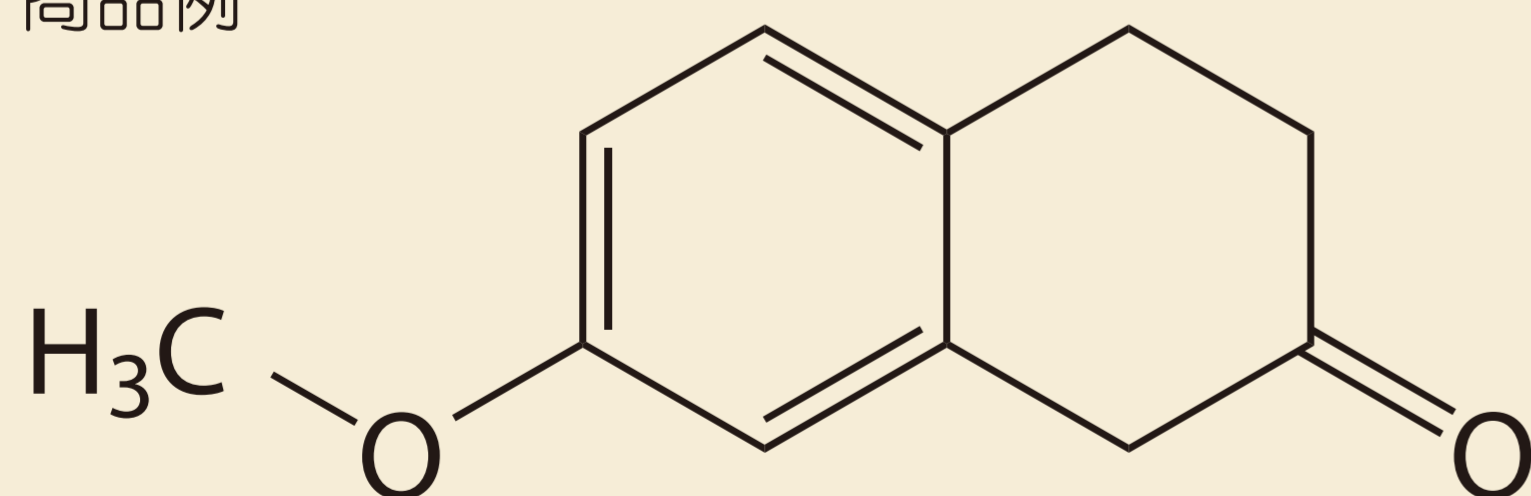
7-Methoxy 2-tetralone
