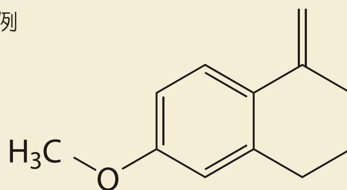
6-Methoxy 1-tetralone
